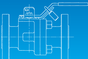
LOCKING DEVICE
