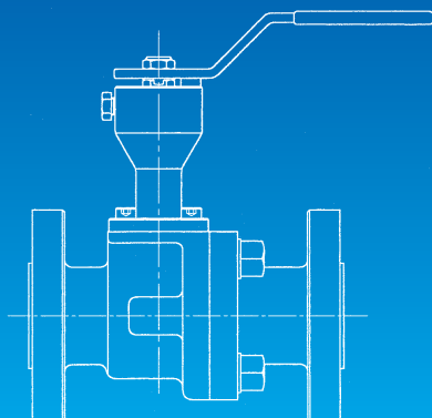
FUGITIVE EMISSION
